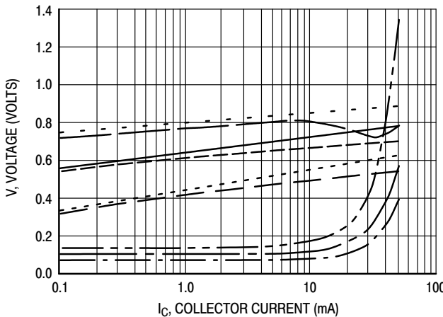
Figure 4. "ON" Voltages
