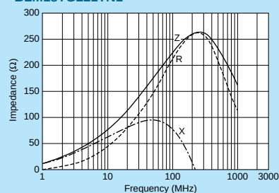
BLM18TG221TN1
